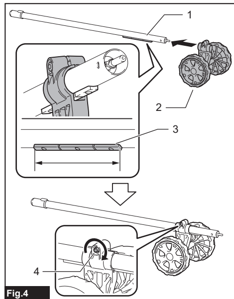
Fig.4 ► 1. Pipe 2. Wheel 3. Plate 4. Bolt
