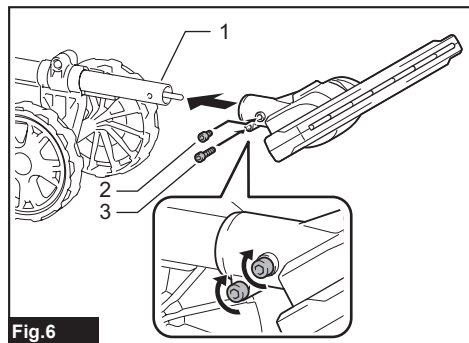
Fig.6 ► 1. Pipe 2. Bolt (short) 3. Bolt (long)
